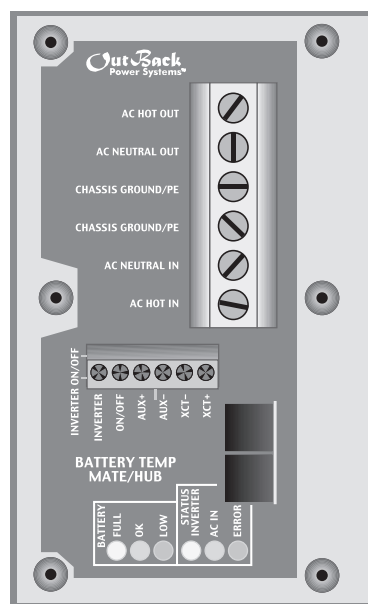
AC Wiring Compartment Board with AUX +/- Terminals
